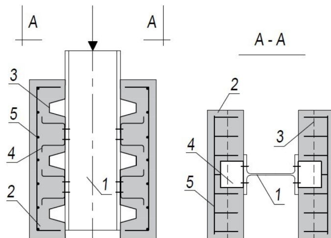
Fig. 2. Test specimen for standard push-out test: 1 – I-beam, 2 – concrete slab, 3 – profiled steel sheeting, 4 – U-shaped connector, 5 – reinforcing bars
