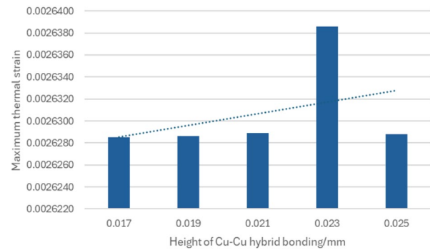
Fig. 6. Maximum thermal strain with different heights of Cu-Cu hybrid bonding
