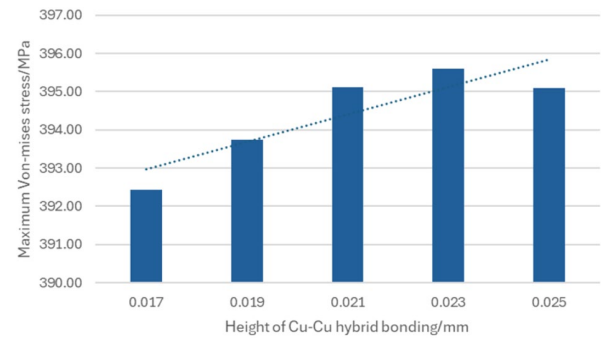
Fig. 7. Maximum Von-mises stress with different heights of Cu-Cu hybrid bonding
