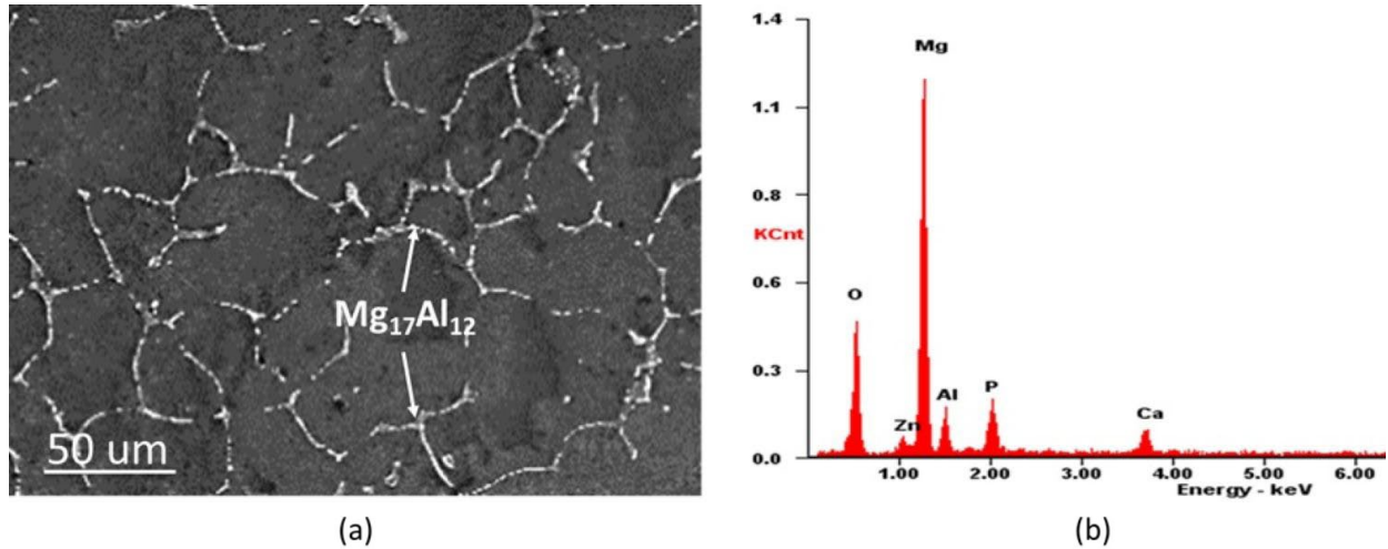
Fig. 4. (a) SEM image of AZ31 Mg alloy and (b) corresponding EDS analysis
