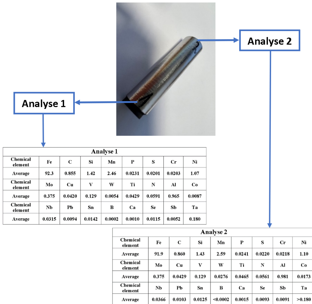
Fig. 1. An example of GDS chemical analysis performed in two places of as cast cylindrical sample
