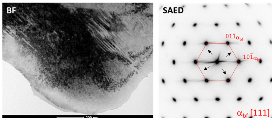
Fig. 8. BF microstructure and the corresponding SAED pattern of bainitic ferrite \alpha_{bf} observed in the sample CS1100
