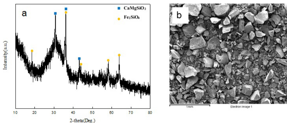
Fig. 1. XRD patterns (a) and SEM-EDS results (b) of the particle of the initial copper slag
