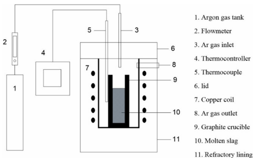
Fig. 2. Schematic diagram of experimental apparatus
