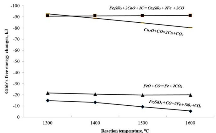
Fig. 4. Gibb's free energy changes of the carbon reduction reaction in the copper smelting slag components
