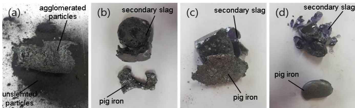
Fig. 5. Smelting behaviour of slag according to reaction temperature (a) 1300°C, (b) 1400°C, (c) 1500°C, and (d) 1600°C
