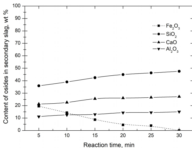
Fig. 7. The content changes of main components in the secondary slag by reaction time
