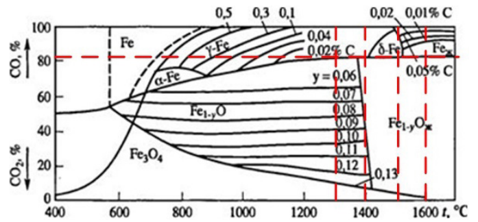
Fig. 3. A diagram of the equilibrium of the systems \text{Fe-O-CO} and \text{C-CO-CO}_2 [17]
