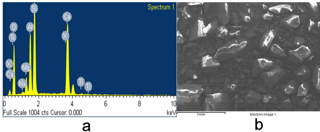
Fig. 6. EDS patterns (a) and SEM results (b) of the particle of the secondary slag
