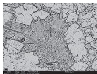
Fig.6. Compacted matrix structure of sinter
