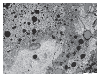
Fig. 5. Typical produced sinter structure
