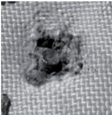
Fig. 5. Front surface of backing with arrested bullet core
