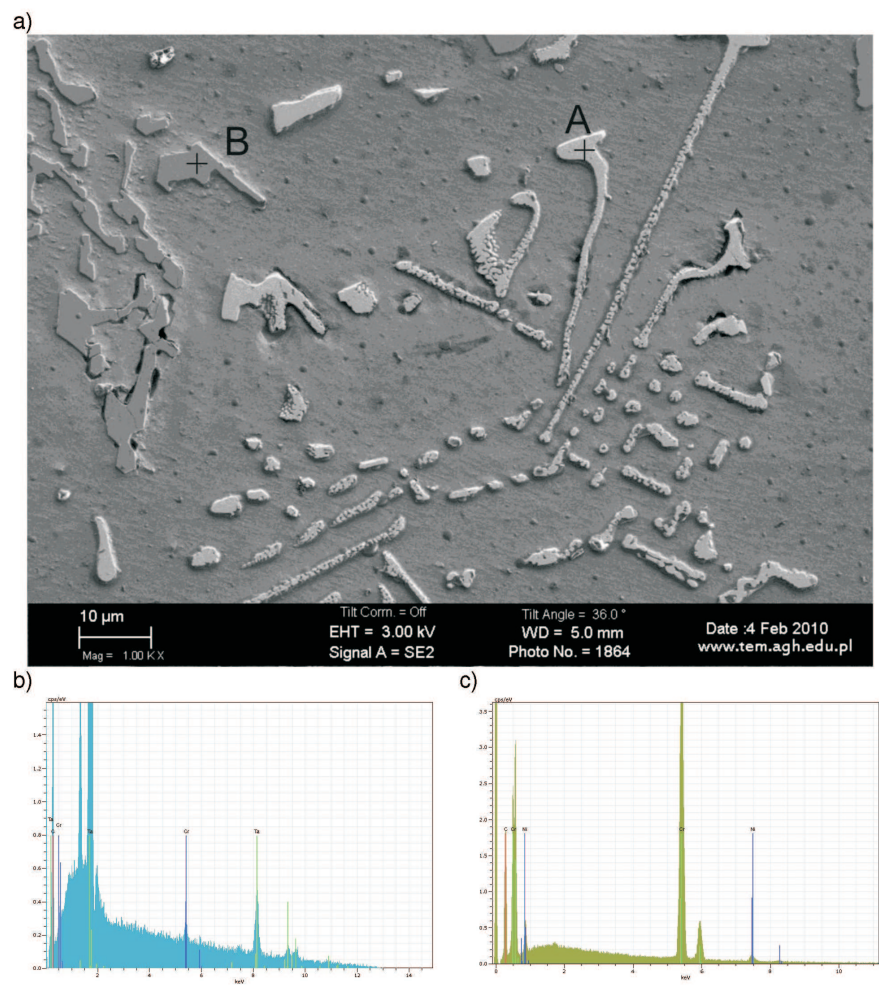
Fig. 4. a) Microstructure of the investigated alloy in as-cast condition with marked zones where from the EDS analysis was performed; b) Characteristic spectrum from A zone; c) Characteristic spectrum from B zone
