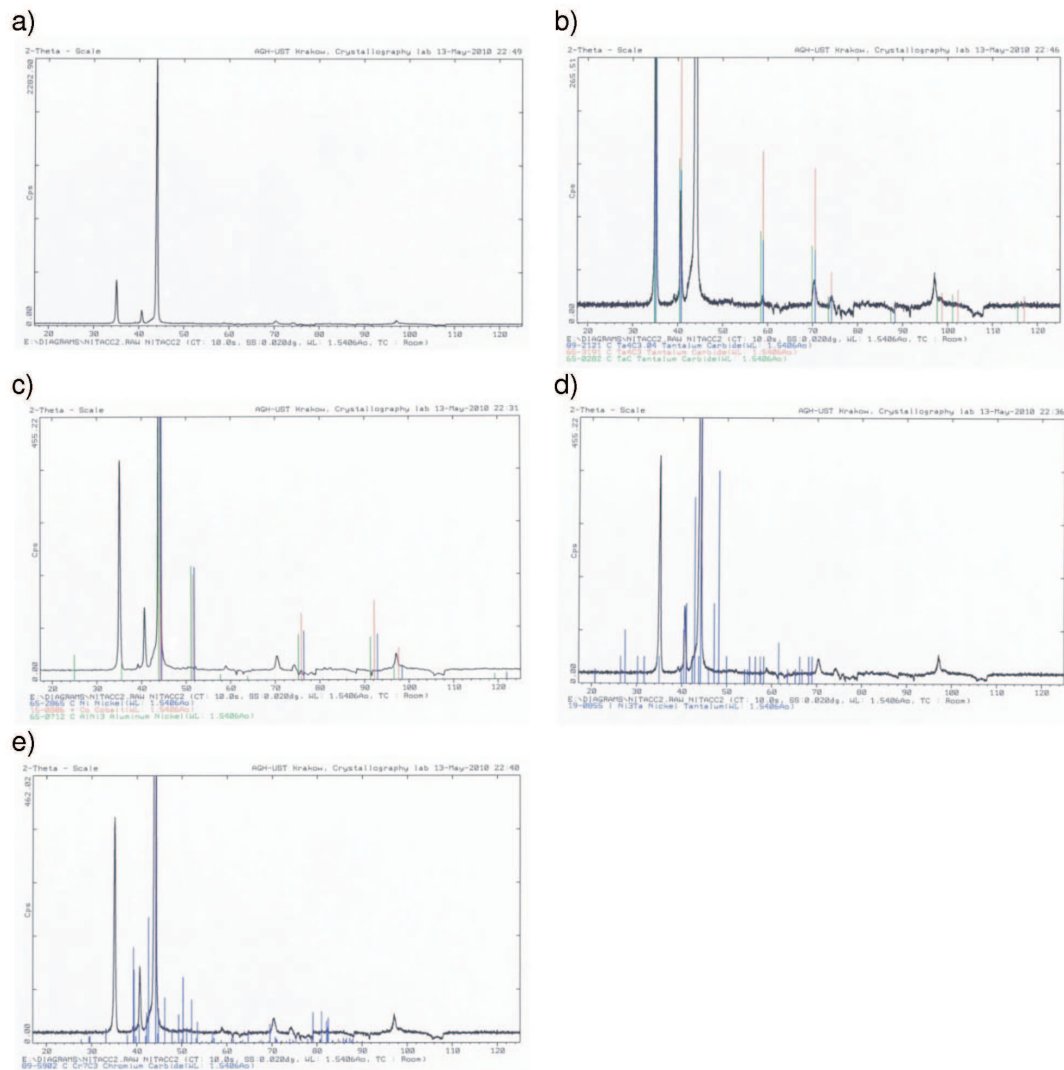
Fig. 5. a) Diffraction, b) Diffraction from Figure a – with lines characteristic for TaC and Ta 4 C 3 carbides, c) Diffraction from Figure a – with lines characteristic for Ni, Co and Ni 3 Al, d) Diffraction from Figure a – with lines characteristic for Ni 3 Ta, e) Diffraction from Figure a – with lines characteristic for Cr 7 C 3 carbide
