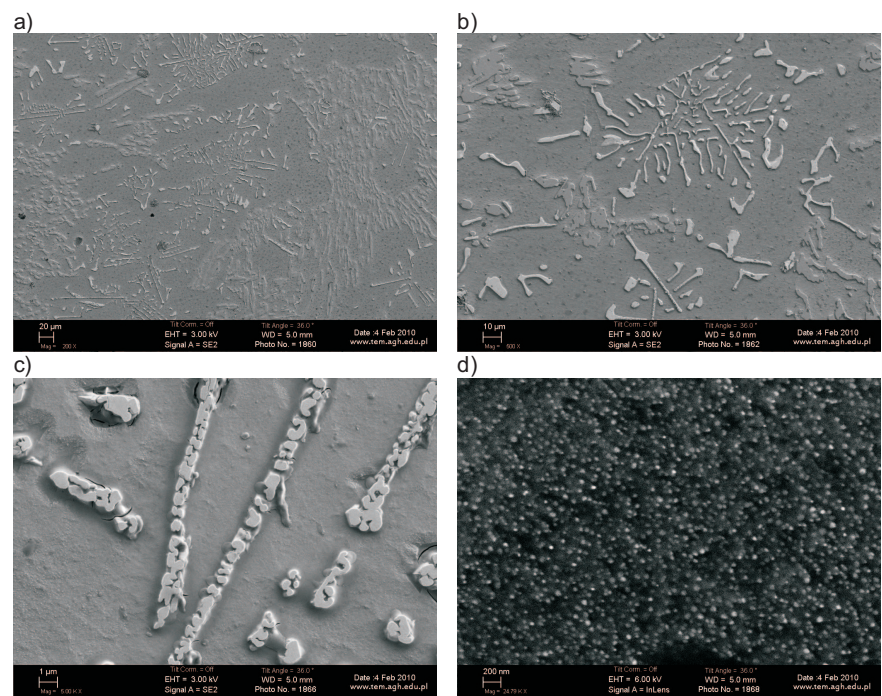
Fig. 3. Microstructure of investigated alloy in as-cast state. SEM
