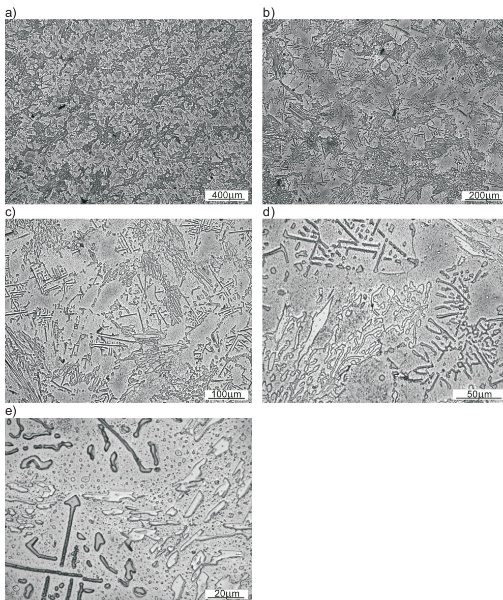
Fig. 2. Microstructure of investigated alloy in as-cast state. Light microscope
