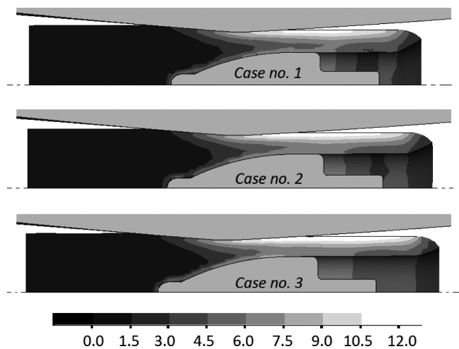
Fig. 11. Effective strain distribution in the semi-finished product obtained in the rotary piercing process (for t \approx 5 s)
