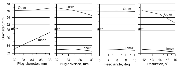
Fig. 16. Effect of the piercing parameters on the diameter dimensions of the tube shells obtained in the piercing process using the Diescher mill
