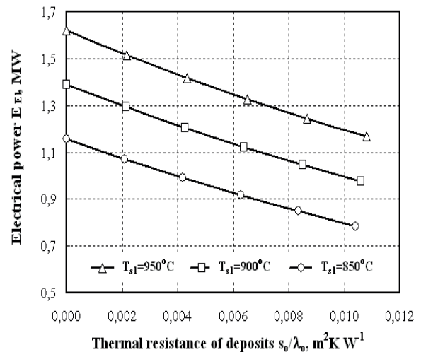
Fig. 5. Electrical power versus thermal resistance of the deposit layer on the tubes
