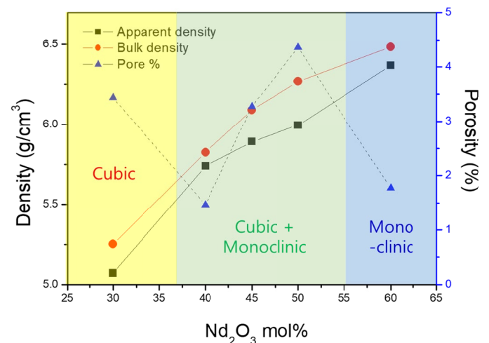
Fig. 4. Summary of the density & porosity of \text{NdYO}_3 with increasing \text{Nd}_2\text{O}_3 contents
