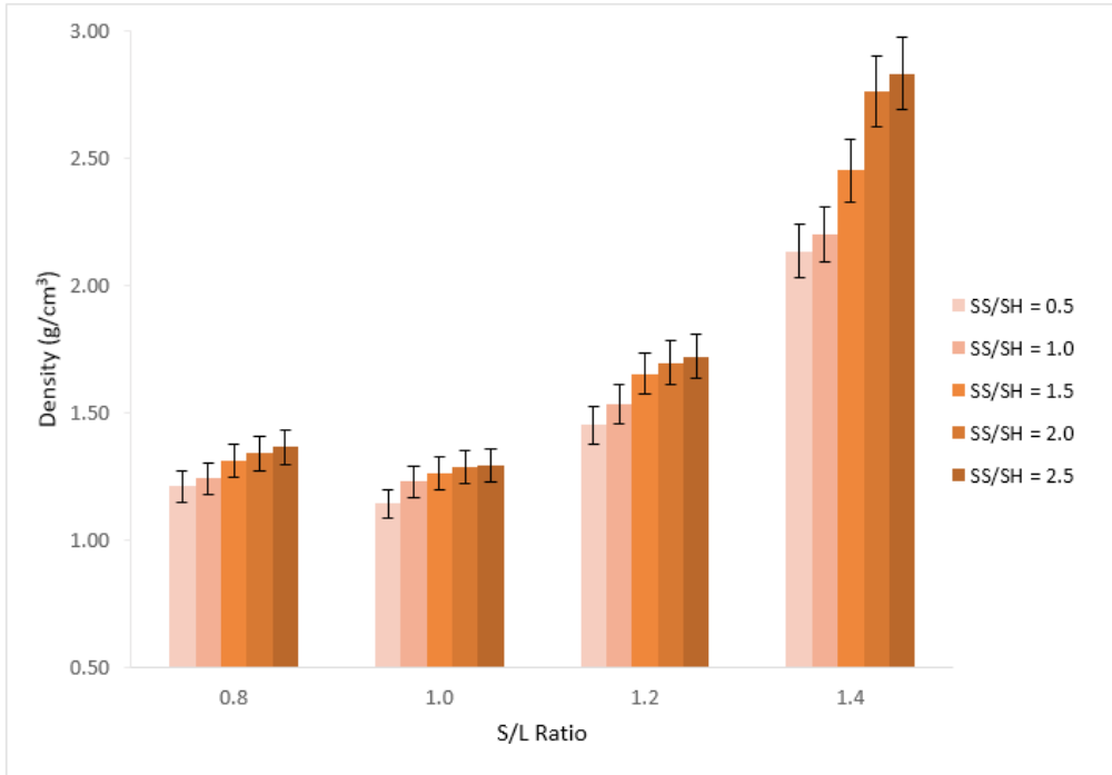
Fig. 2. Density of metakaolin membrane geopolymer with different S/L and Na 2 SiO 3 /NaOH proportion
