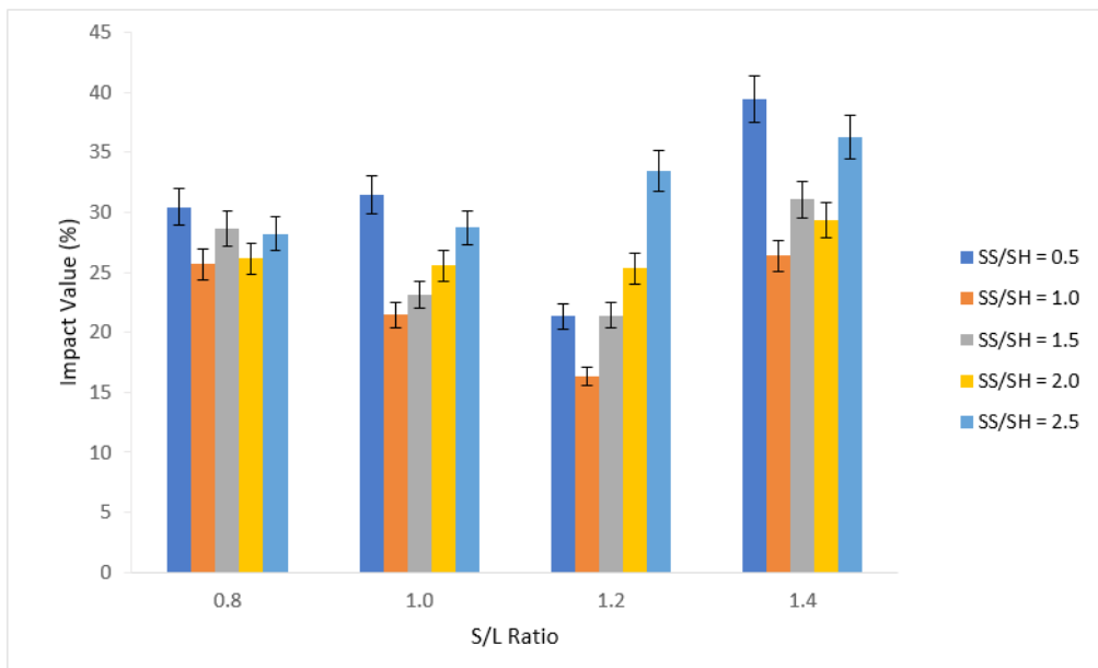
Fig. 3. Impact value of metakaolin membrane geopolymer with different S/L and Na 2 SiO 3 /NaOH ratio
