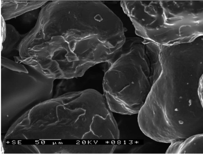
Fig. 1. Film of glassy sodium silicate covering grain surfaces of high-silica matrix of core sand used in manufacture of cast-steel castings
