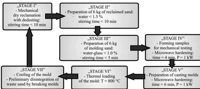
Fig. 4. Schematic presentation of modified processing cycle of waste molding sand carried-out in laboratory conditions
