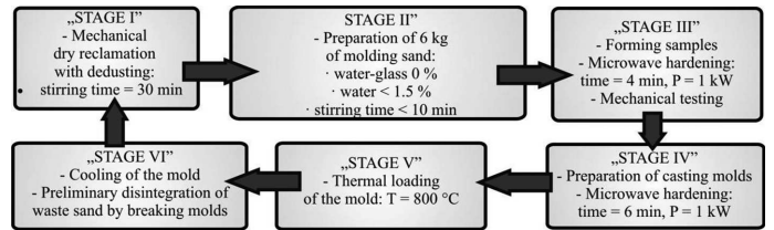
Fig. 2. Schematic presentation of one processing cycle of waste molding sand carried-out in laboratory conditions
