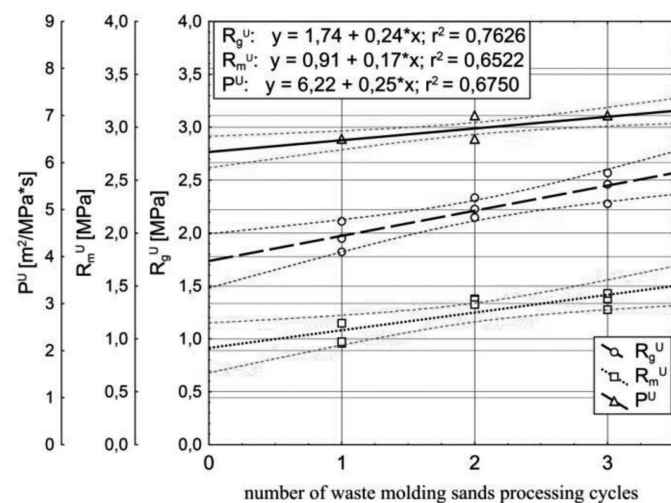
Fig. 5. Diagram of permeability and strength changes controlled at "Stage IV" of three processing cycles of waste molding sand
