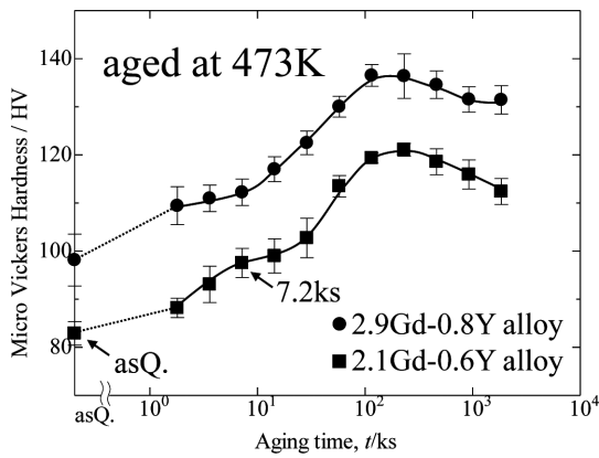
Fig. 1. Age-hardening curves of 2.9Gd-0.8Y alloy and 2.1Gd-0.6Y alloy aged at 473K
