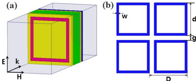
Fig. 1. Schematic description of (a) SL-FSS on grounded ferrite composite and (b) its dimension ( D = 10 mm, d = 8.75 mm, w = 0.625 mm, g = 0.625 mm)
