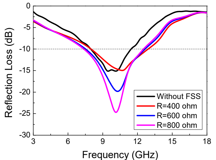
Fig. 4. Reflection loss determined in the composite structure, implemented with SL-FSS on a grounded ferrite composite (thickness = 2.9 mm), with increasing SL-FSS resistance ( R )
