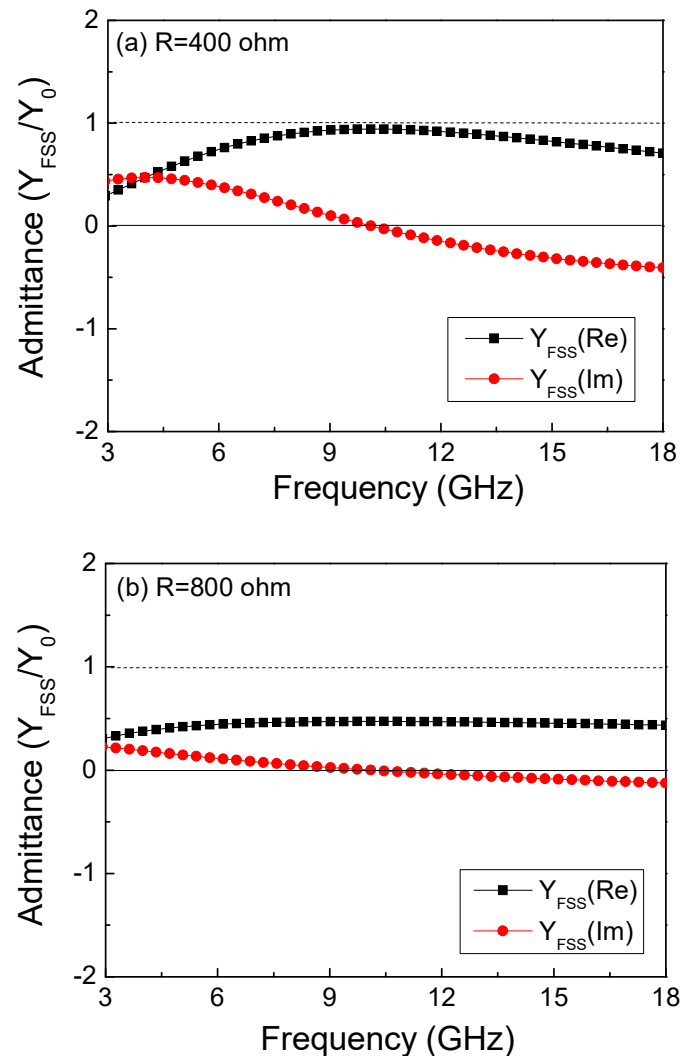
Fig. 6. Normalized real and imaginary parts of complex admittance of SL-FSS with varying varying SL-FSS resistance: (a) R = 400 \Omega , (b) R = 800 \Omega
