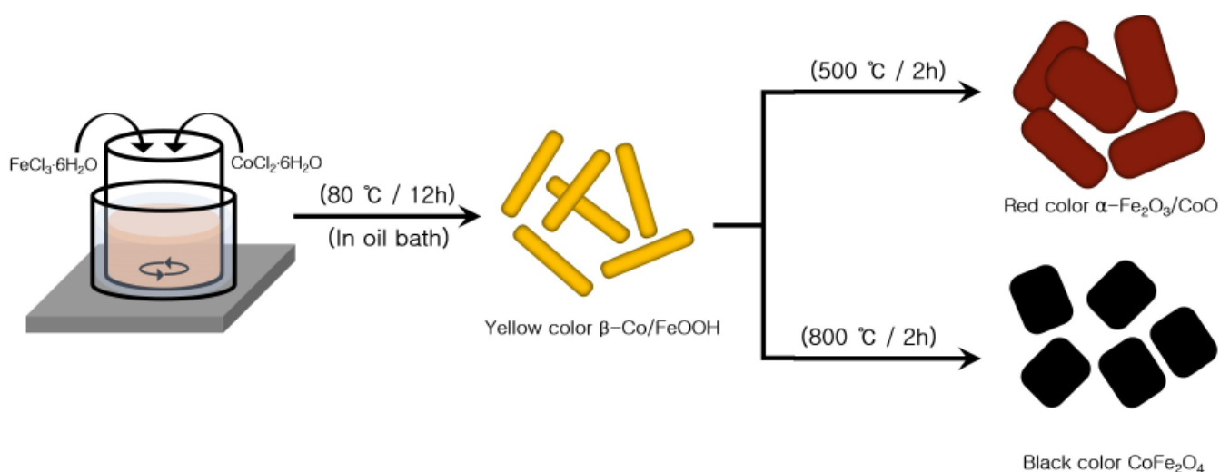
Fig. 1. Schematic illustration of the formation of the CoFe 2 O 4 black pigment with heat-treatment
