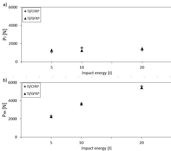
Fig. 3. P_i (a) and P_m (b) values vs. impact energy and type of laminate.
