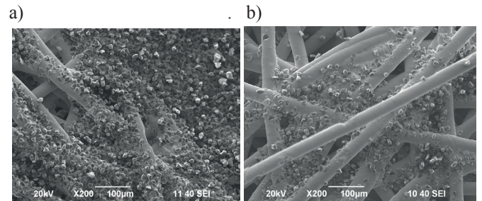
Fig. 4: SEM images of the surface of Ni-P composite coatings with D 14/20 μm deposited under: a) regime “a”; b) regime “f” (0.01 g/l SLS; T = 82 °C; τ = 60 min)
