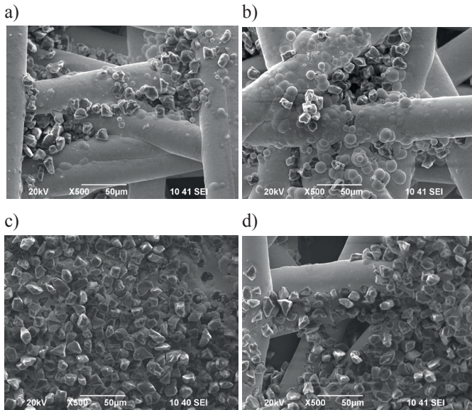
Fig. 2: SEM images of the surface of composite Ni-P composite coatings obtained at different concentrations of D 14/20 μm: a) 1.0 g/l; b) 2.5 g/l; c) 5.0 g/l; d) 10.0 g/l (0.01 g/l SLS; T = 82 °C; τ = 60 min; continuous stirring)
