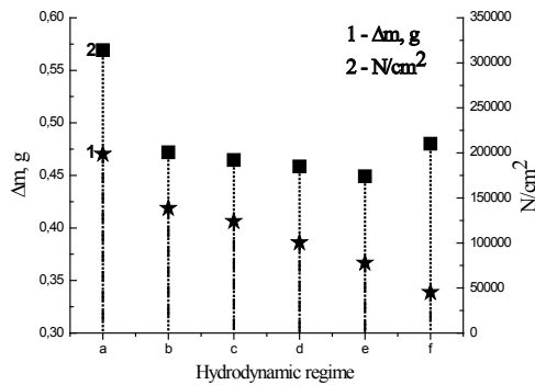
Fig. 3: Influence of the hydrodynamic regimes on the mass and number of co-deposited particles in composite coatings (0.01 g/l SLS; T = 82 °C; τ = 60 min)
