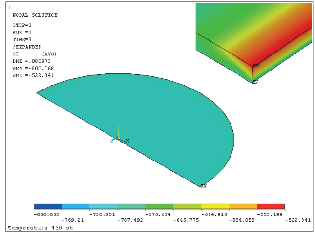
Fig. 1. Distribution of the simulated compression stresses in the TiN coating (coating thickness g=3.9 μm, process temperature 460°C)
