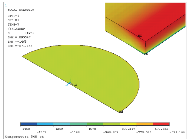
Fig.2. Distribution of the simulated compression stresses in the TiC coating (coating thickness g=2.6 μm, process temperature 540°C)
