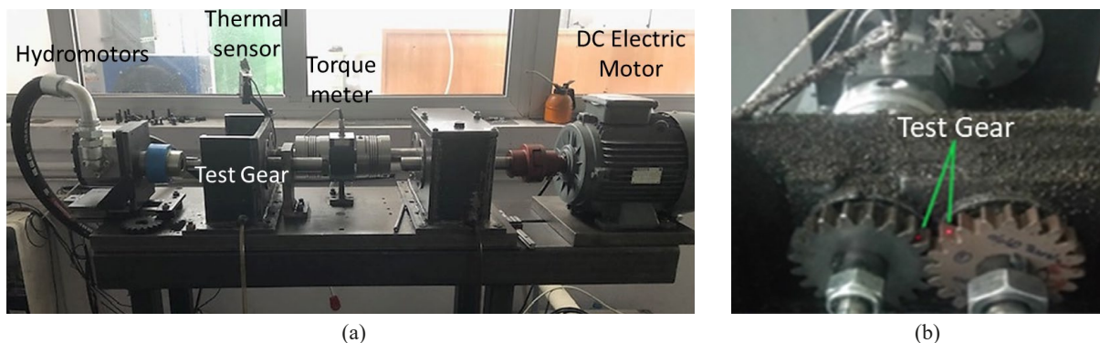
Fig. 2. Gear tester, a) test device, b) non-contact temperature measuring device
