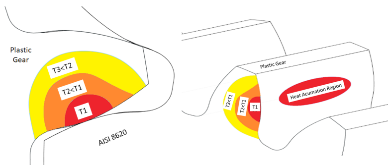
Fig. 1. Heat accumulation zones of plastic gear [2,20]
