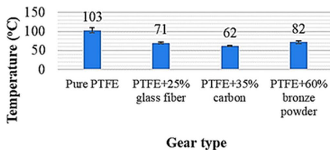
Fig. 7. Highest temperature values measured during the test
