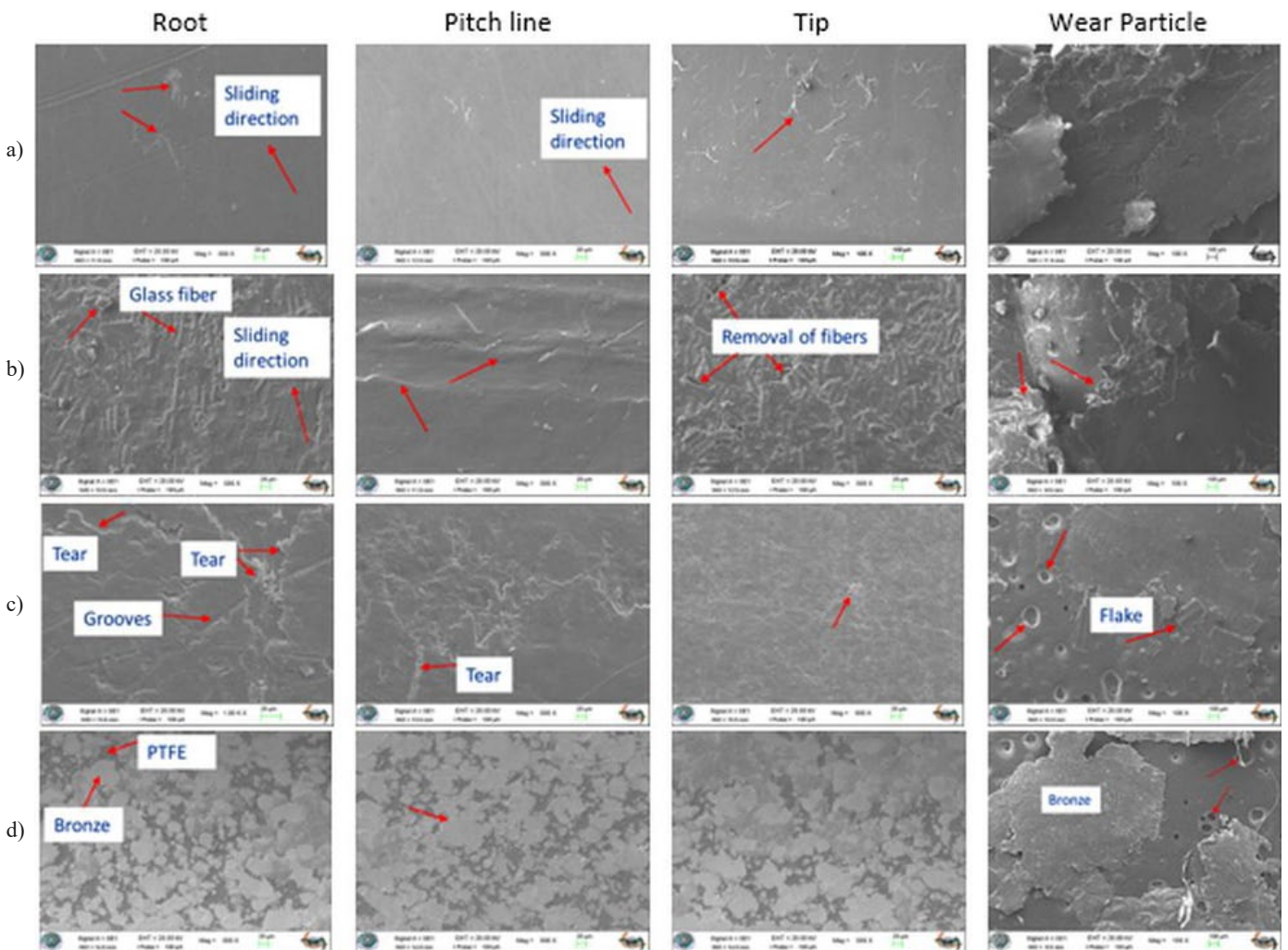
Fig. 9. SEM images of the root, pitch region, tip, and wear particles after the test, a) pure PTFE, b) PTFE+25% glass fiber, c) PTFE+ 35% carbon, d) PTFE+60% bronze powder
