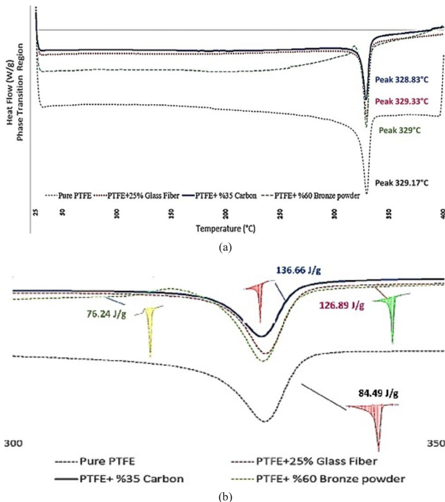
Fig. 3. Thermal traces of PTFE and PTFE composites, determined with DSC, a) heat of fusion and melting peak, b) heat of fusion in the range of 300-350 ^{\circ}\text{C}
