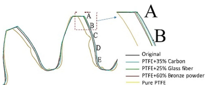
Fig. 6. 2D wear depth in the tooth profile
