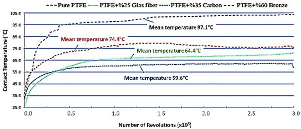
Fig. 8. Change in tooth temperature in the contact zone of the gear during the test
