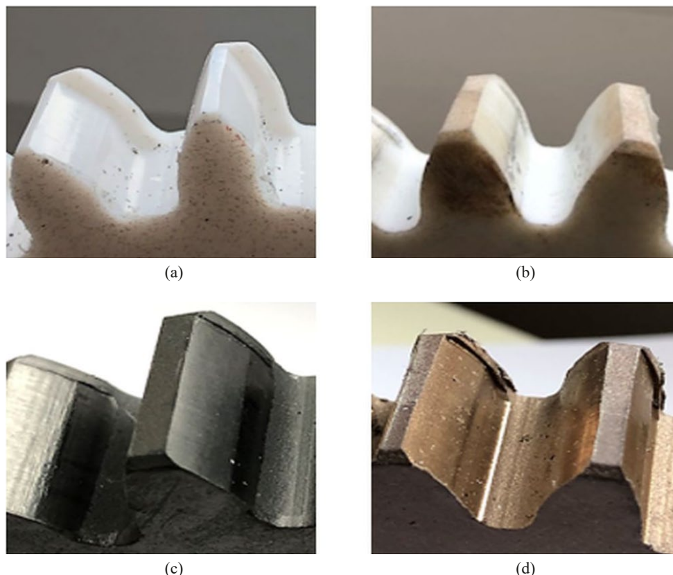
Fig. 5. Wear in the tooth contact areas of PTFE composite gears, a) pure PTFE, b) PTFE+25% glass fiber, c) PTFE+35% carbon, d) PTFE+60% bronze powder gears
