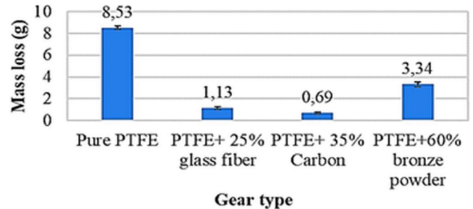
Fig. 4. Test gear wheels, mass losses after testing
