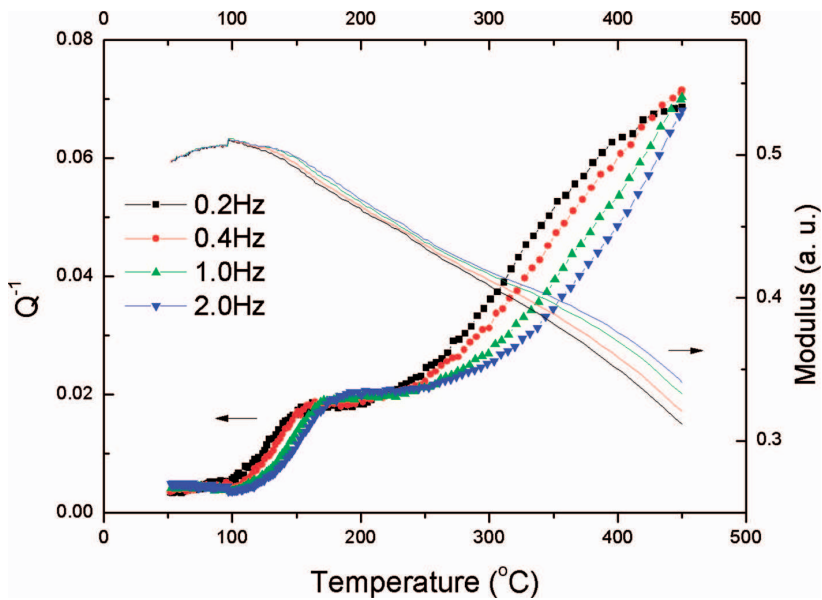
Fig. 7. Internal friction and relative modulus of pure Mg bicrystals with 25.0° [0001] grain boundaries. The specimen dimensions are 60 mm×2 mm×2 mm, so the grain boundary density of the bicrystal is twice as that of the bicrystal in Fig. 5
