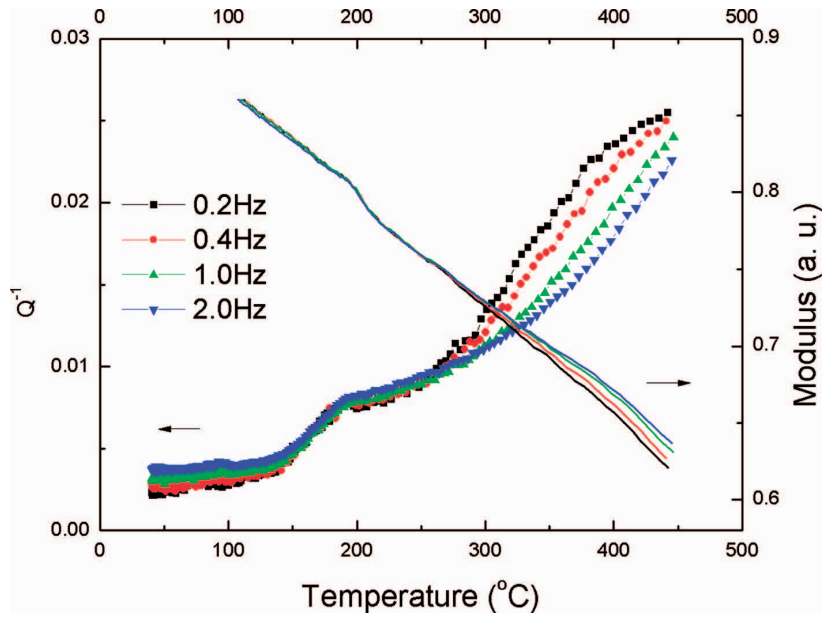
Fig. 6. Internal friction and relative modulus of pure Mg bicrystals with 38.0° [0001] symmetric tilt grain boundaries
