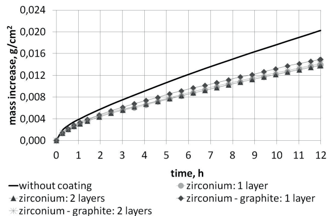
Fig. 4. Proceeding of the moisture sorption from surroundings by surface layers of moulds made of furan moulding sands on the reclaimed sand grains
