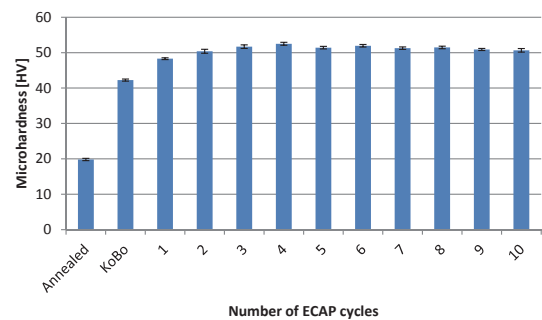
Fig 9. Vickers microhardness for samples in the annealed condition and after KoBo and ECAP processing
