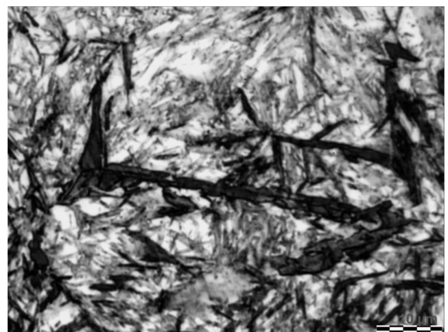
Fig. 7. Observation of microstructure details with visible lower bainite accelerated by small amounts of prior athermal martensite after austempering with isothermal transformation at 160°C during 3 min., etching with nital
