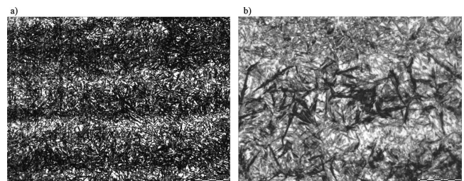
Fig. 6. Microstructure heterogeneity for steel 100CrMnSi6-4 caused by carbide banding along rolling after isothermal austempering at 160°C during 540s a) secondary banding as a result of matrix austempering diversity, b) enlarged fragment of the microstructure image within martensitic and bainitic matrix (etching by nital), banding size 7.3 by Stahl-Eisen-Prüfblatt SEP 1520 (4% nital etching)
