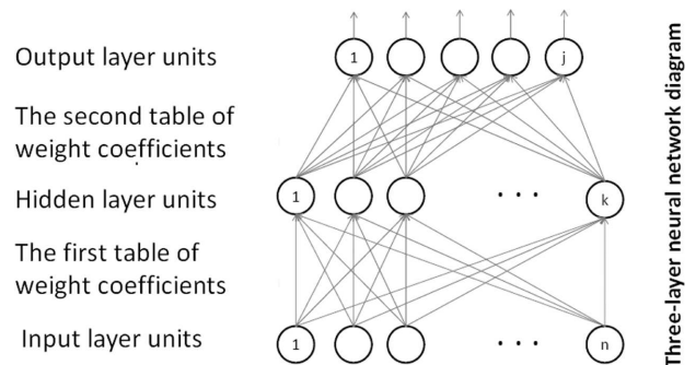
Fig. 4. Neural network learning of acoustic emission neural signals
