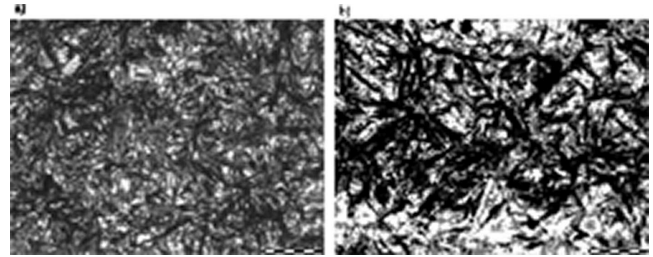
Fig. 5. Image of microstructure after austempering with isothermal transformation at 160°C a) during 8400s etched lower bainite accelerated by small amounts of prior athermal martensite (4% nital etching), b) during 240 s, the image after digital processing with visible plates of lower bainite accelerated by small amounts of prior athermal martensite in black colour, bainite in grey and residual austenite in white
