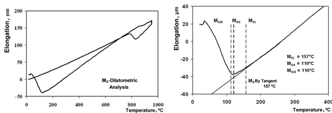
Fig. 8. Dilatometry results: a) example of dilatometric curves, b) fragment of the curve from fig. a) during cooling, with marked characteristic points
