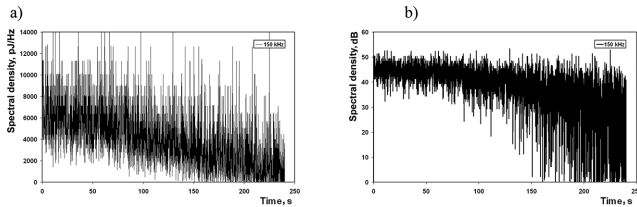
Fig. 11. Exemplary components of tested acoustic emission band from digital filtration for frequency of 150 kHz against time a) pJ/Hz, b) dB. Isothermal quenching at temperature 160°C
