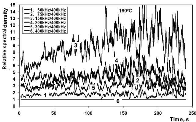
Fig. 12. Relative values of the components of the signal spectrum defined by digital filtering during isothermal quenching at 160°C, curves were drawn for arithmetic means from each 30 consecutive measurements (moving average)
