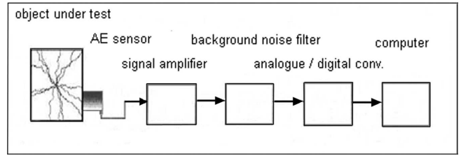
Fig. 2. Block diagram of the stand for testing acoustic emission, broad-band sensor of WD type (20 kHz–900 kHz), card ADLINK 9812 with frequency 1,200 kHz, data format bipolar mode 5V, RMS value of the noise at the input of the preamplifier was app. 12-15 microvolts, after amplifying 2.000 times (66 dB) 24 mV
