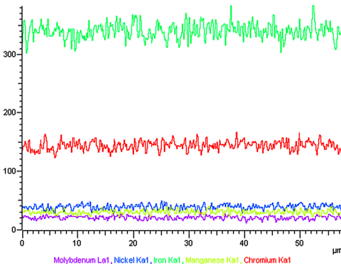
Fig. 10. Energy Dispersive X-ray Spectroscopy analysis of friction welded joint
