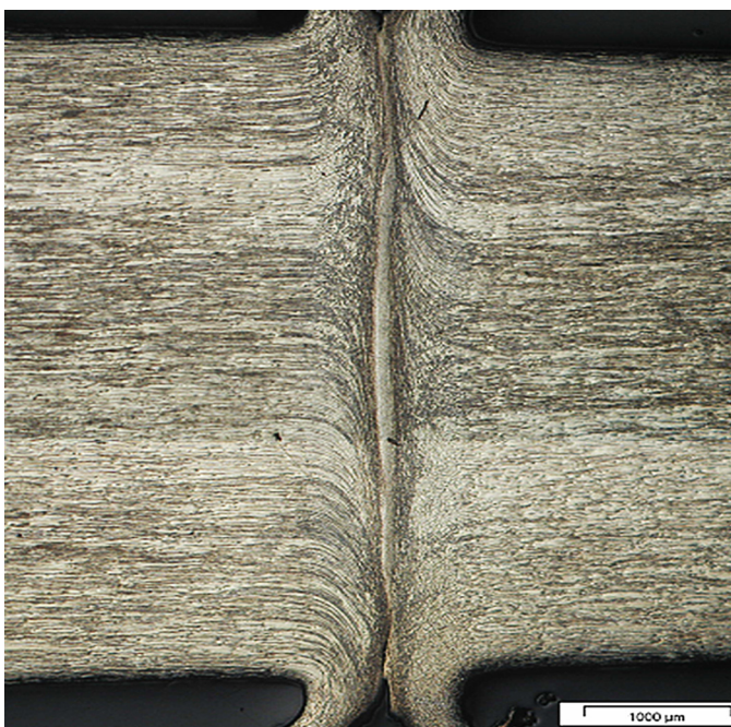
Fig. 7. Microstructure of friction welded joint of 316L UFG steel, etched
