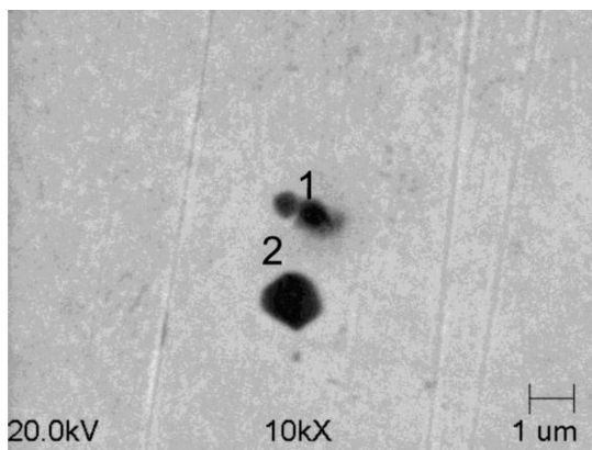
Fig. 8. Non-metallic inclusions in the metal bath in ladle furnace (LF)
