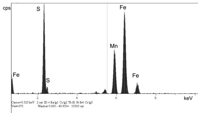
Fig. 10. X-ray spectrum with the energy dispersion (EDS) – from point 2 in Fig. 8
