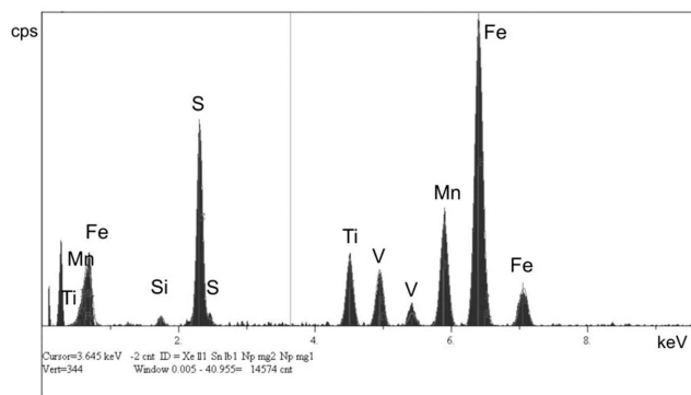
Fig. 9. X-ray spectrum with the energy dispersion (EDS) – from point 1 in Fig. 8
