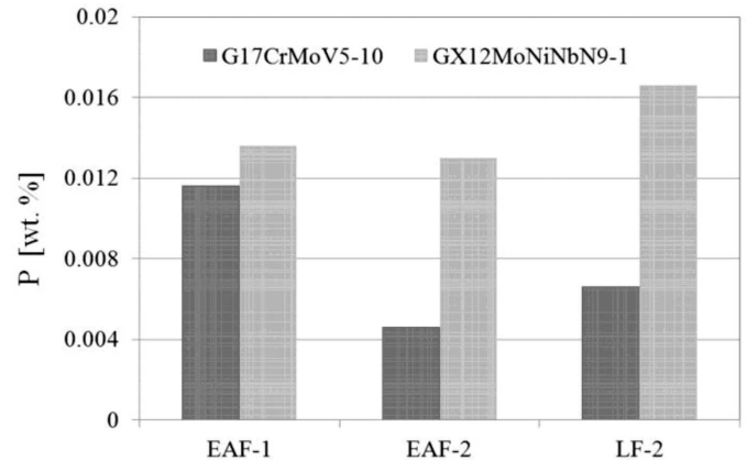
Fig. 3. Changes of the P content during the steel melting in the process EAF+LF
