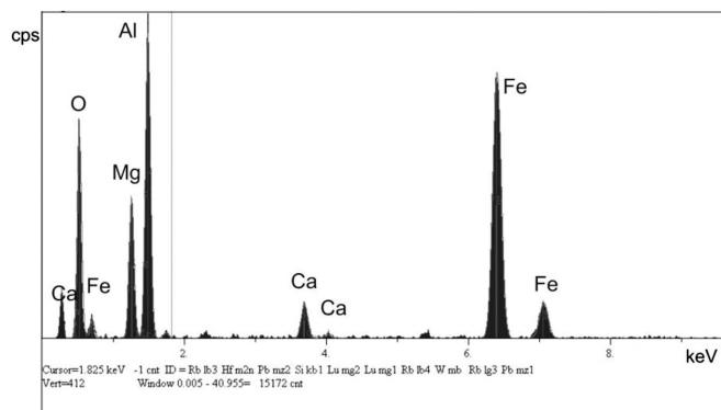
Fig. 7. X-ray spectrum with the energy dispersion (EDS) – from point 2 in Fig. 5
