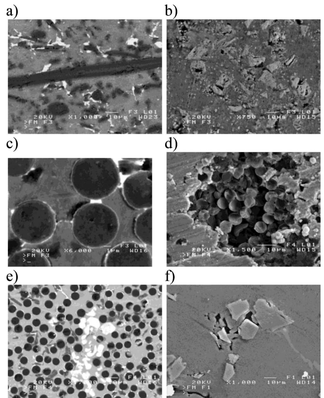
Fig. 1. Microstructure of metal matrix composite castings (SEM): a, b – fractures (damage of reinforcing phase); c, d – insufficient saturation of reinforcing phase with matrix metal; e, f – inhomogeneity of arrangement and size of the reinforcing phase
