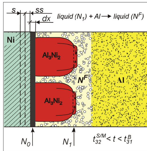
Fig. 7. Reaction for the N^F – equilibrium solution formation; arrows located in the neighborhood of the N_1 – solute concentration indicate the liquid which remains at the Al_3Ni_2 – cells front after the first peritectic transformation (during initial transient stable solidification); next, situations of the s – saturation zone and ss – super-saturation zone in the Ni – substrate are distinguished according to Fig. 6
