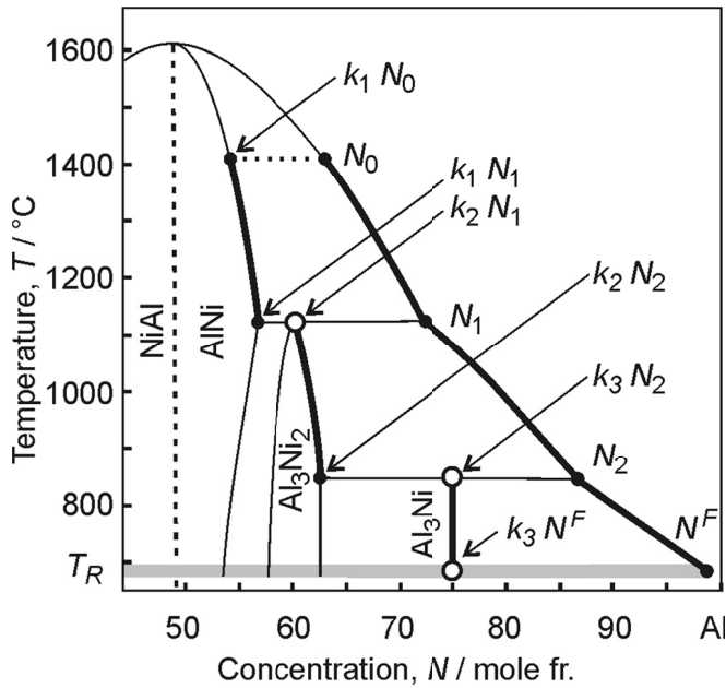
Fig. 3. Situation of the N_0 = N_{\min} – solute concentration in the Ni-Al phase diagram for stable equilibrium according to the mass balance in the system: liquid(N_0)/diffusion\ barrier(\bar{N} = N_0)
