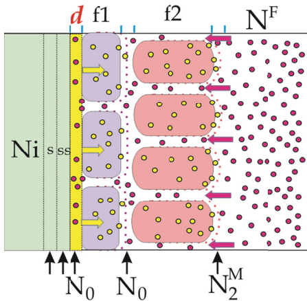
Fig. 11. Model for the ideal formation of the diffusion barrier within the Ni/Al – nano-foil; d \equiv dx is the dissolution zone within the Ni – substrate; the red arrows show the direction of the boundary diffusion of the N^F – solution towards the Ni-substrate; the yellow arrows show the direction of the bulk diffusion of the N_0 – liquid from the d \equiv dx zone to the f1 \equiv \text{Al}_3\text{Ni}_2 – phase front; the N_2^M – remaining liquid diffuses to the front of the f2 \equiv \text{Al}_3\text{Ni} – compound
