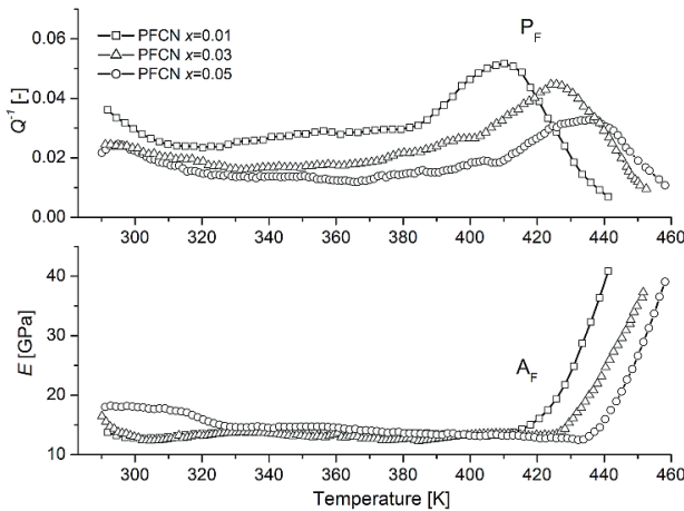
Fig.2. Temperature relationships of the Q^{-1}(T) internal friction and the E(T) dynamic Young's modulus of the admixed PCFN ceramics for x = 0.01, 0.03 and 0.05 ( f = 753 Hz).
