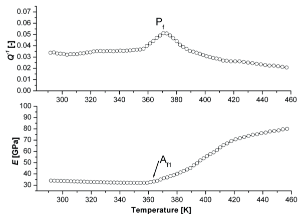
Fig.1. Temperature relationships of the Q^{-1}(T) internal friction and the E(T) dynamic Young's modulus for the non-admixed PFN ceramics ( f = 760 Hz)
