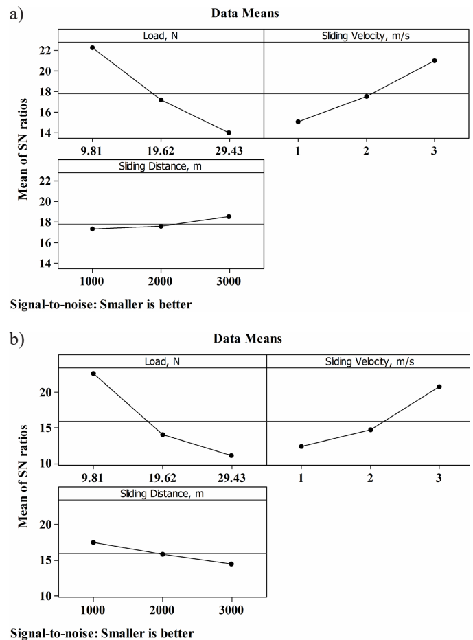
Fig. 3. Optimal plot for: (a) specific wear rate; (b) coefficient of friction
