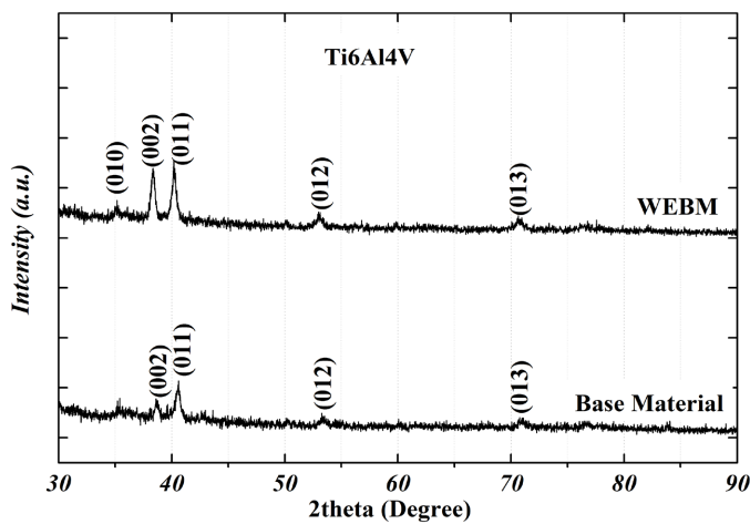
Fig. 1. X ray diffraction of additive sample
