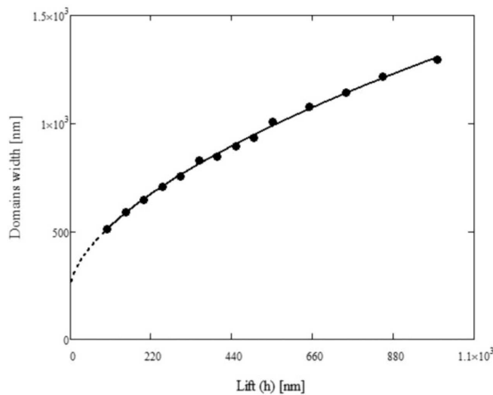
Fig. 8. Changes in FWHM widths vs. lift height (closed points) best fitted with the power function (solid line) and its extrapolation down to zero lift height (dotted line)
