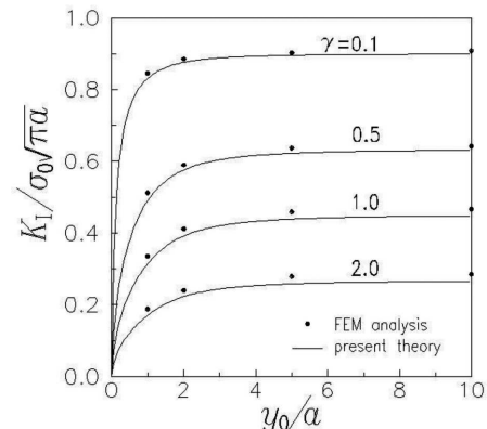
Fig. 3. Dimensionless stress intensity factors as a function of the seam welding location and the stiffness ratio
