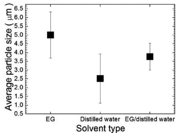
Fig. 6. Size distribution of Cu powders synthesized in 3 h at 90°C with different solvent types (the added amount of L-ascorbic acid was 272.8 mM)
