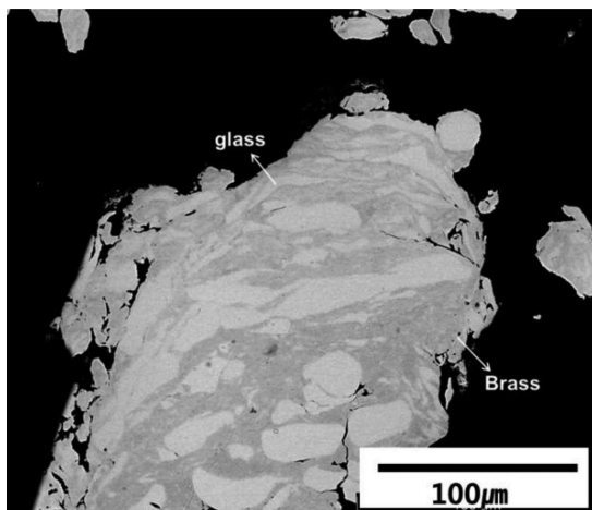
Fig. 1. Cross sectional image of Ni-based metallic glass powders
