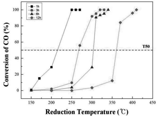
Fig. 2. Conversion of CO vs. Reduction temperature of Ni-based porous powders
