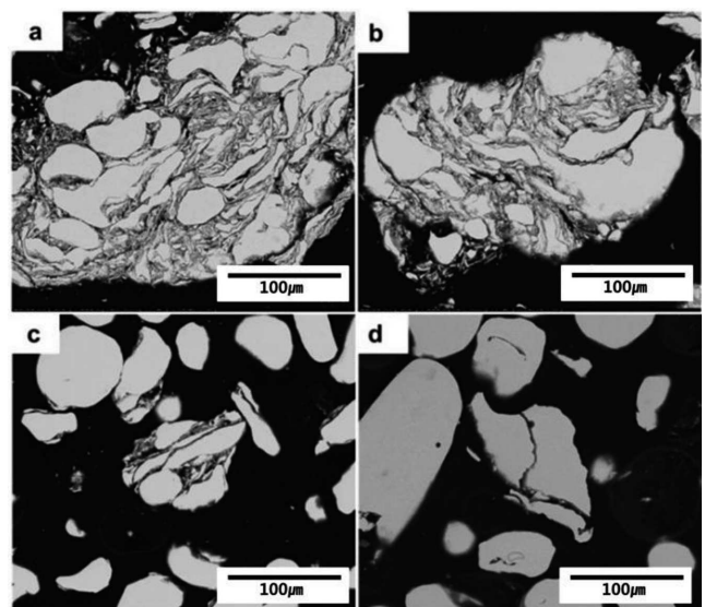
Fig. 3. SEM backscattered electron images obtained from the polished cross section of the porous powder;(a)1h, (b)3h, (c) 6h, (d) 12h
