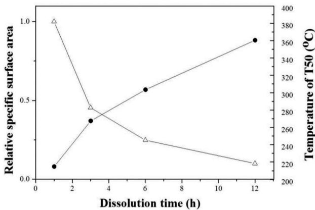
Fig. 4. Relative specific surface area and temperature of T50 vs. dissolution time
