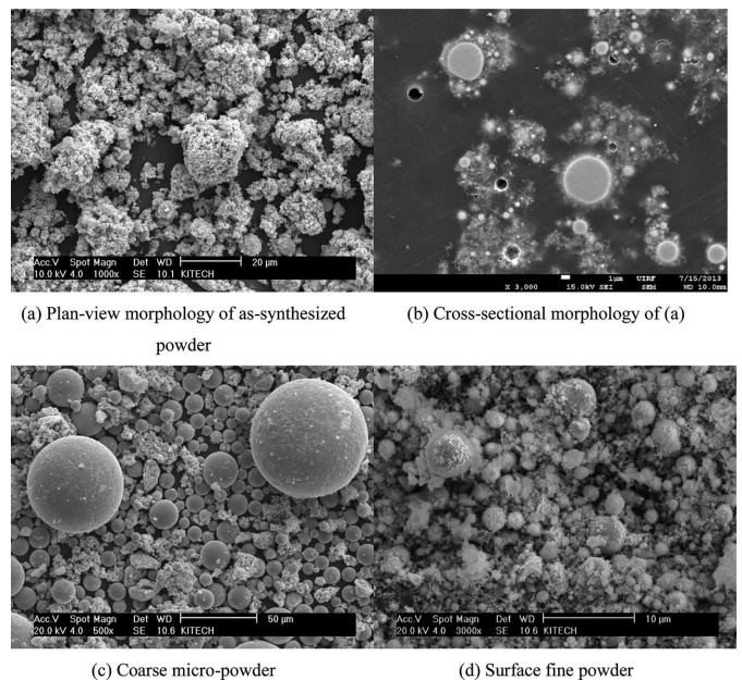
Fig. 1. Morphologies of as-synthesized 316L stainless steel powder, coarse micro-powder, and surface fine powder. Coarse micro-powder and surface fine powder are obtained from ultrasonic detachment of the synthesized powder: (a) Plan-view morphology of as-synthesized powder, (b) Cross-sectional morphology of (a), (c) Coarse micro-powder and (d) Surface fine powder
