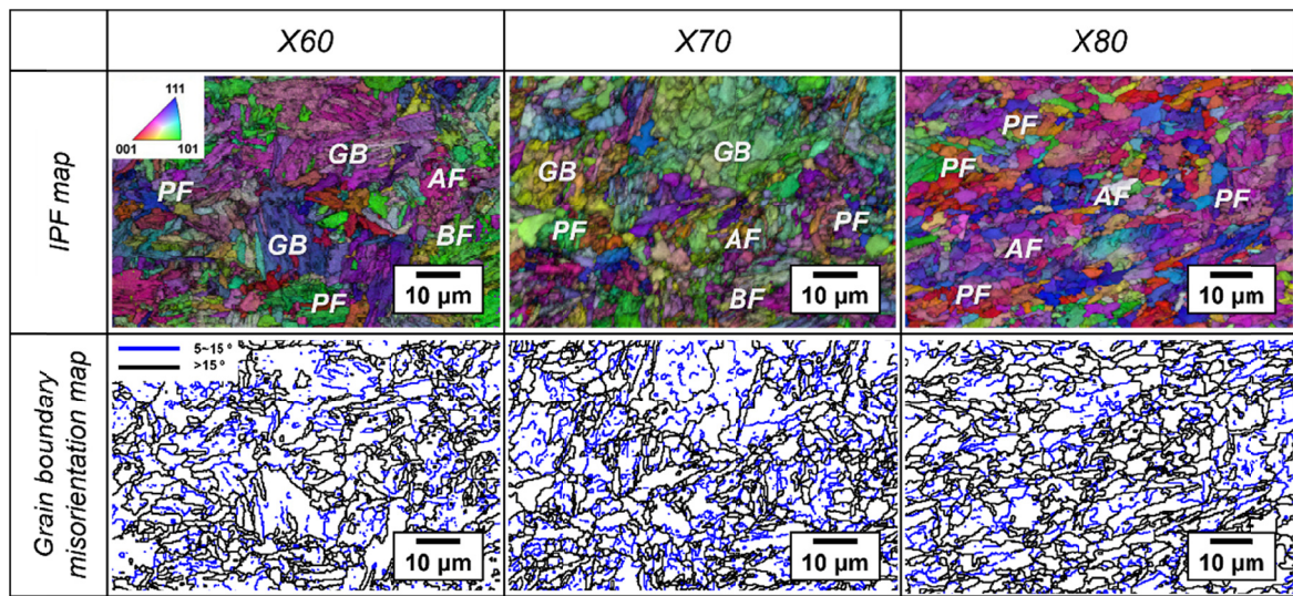
Fig. 2. Electron backscatter diffraction (EBSD) inverse pole figure (IPF) and grain boundary misorientation maps of the API X60, X70, and X80 pipeline steels [11]. Longitudinal-transverse (L-S) planes are observed. Polygonal ferrite (PF), acicular ferrite (AF), granular bainite (GB), and bainitic ferrite (BF) are marked in IPF maps. In grain boundary misorientation maps, the angle ranges of blue and black lines are 5 \sim 15^\circ , and >15^\circ , respectively. The grain size and fraction of the high-angle grain boundary of the API X60, X70, and X80 pipeline steels were calculated to be 20.5 \mu\text{m} and 4.3%, 17.6 \mu\text{m} and 6.0%, and 16.1 \mu\text{m} and 7.8%, respectively
