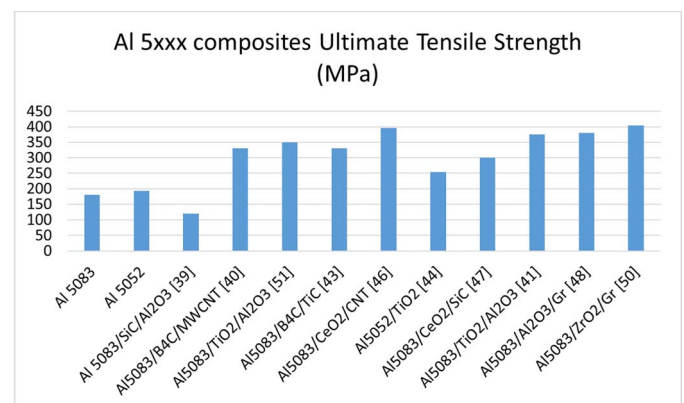
Fig. 4. Ultimate tensile strength of Al 5xxx hybrid surface composites
