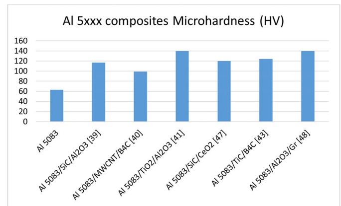
Fig. 3. Microhardness (HV) values of Al 5xxx hybrid surface composites
