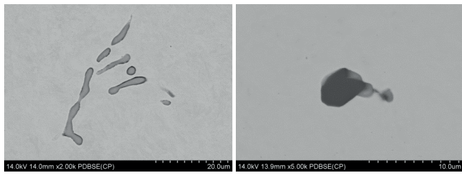
Fig. 10. Morphology of the non-metallic precipitates from the cast steel ingot (SEM)
